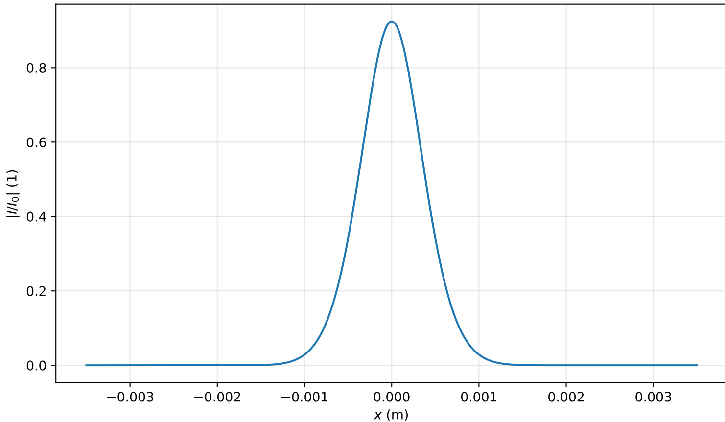
Intensity profile I(x, y = 0, z = 1.035m)/I_0 , P_{in}=0.3P_{cr} , artificial time
